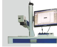
Fiber Laser Printer/Online 20W, 75x75 to 300x300mm, 8000mm/s
